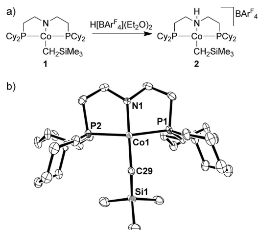
Scheme 1. a) Complexes 1 and 2. b) X-ray structure of complex 1 (thermal ellipsoids at 50% probability, hydrogen atoms omitted for clarity). Two crystallographically independent molecules were present in the unit cell for complex 1, one of which is shown above. Selected bond distances [Å] and angles [°]: Co1–N1 1.880(3), Co1–P1 2.202(1), Co1–P2 2.204(1), Co1–C29 2.005(3); N1–Co1–C29 172.2(1), N1–Co1–P1 84.9(1), C29–Co1–P1 95.4(1), N1–Co1–P2 84.6(1), C29–Co1–P2 95.7(1), P1–Co1–P2 168.7(4).
